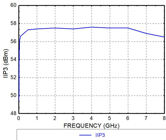
IIP3 (10MHz~7GHz)
